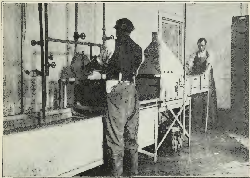
FIG. 19.—Turbine-brush bottle washer. Bottles are rinsed by sprays of boiling water forced into them by pump.
